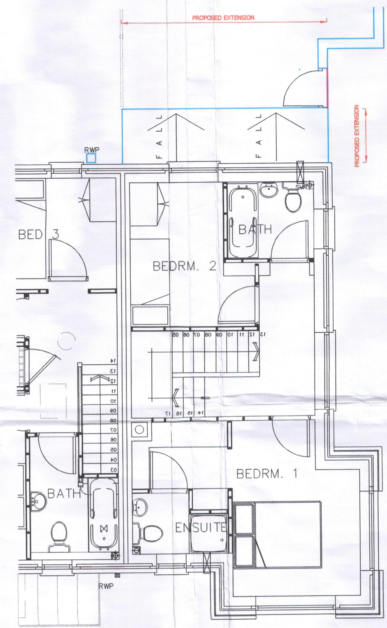
FRST FLOOR PLAN
